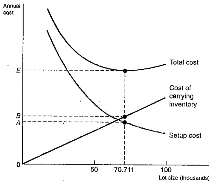
FIGURE 3. Relationship between Size of Lot and Total Annual Costs. Total cost is the sum of the cost of carrying inventory and the setup cost. Thus the "Total cost" curve is the vertical sum of the "Cost of carrying inventory" curve and the "Setup cost" curve. For example, if the Lot size is 70,711, annual setup cost equals OA , annual inventory cost equals OB , and annual total cost equals OA + OB = OE .
