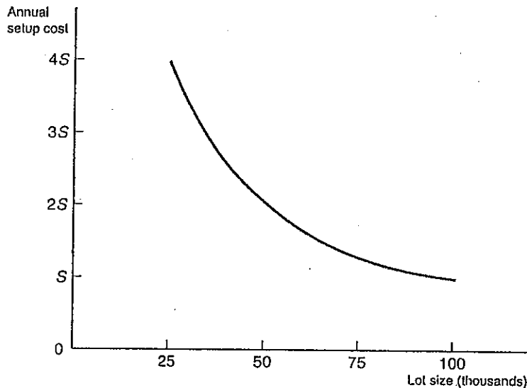
FIGURE 1. Relationship between the Size of Lot and the Annual Setup Costs. The larger the lot size, the lower the annual setup costs.
