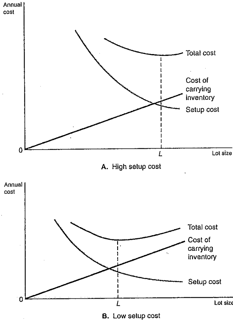
FIGURE 4. Effect of Cost per Setup on Optimal Lot Size. If the cost per setup is relatively high (as in panel A), the optimal lot size tends to be relatively large.
