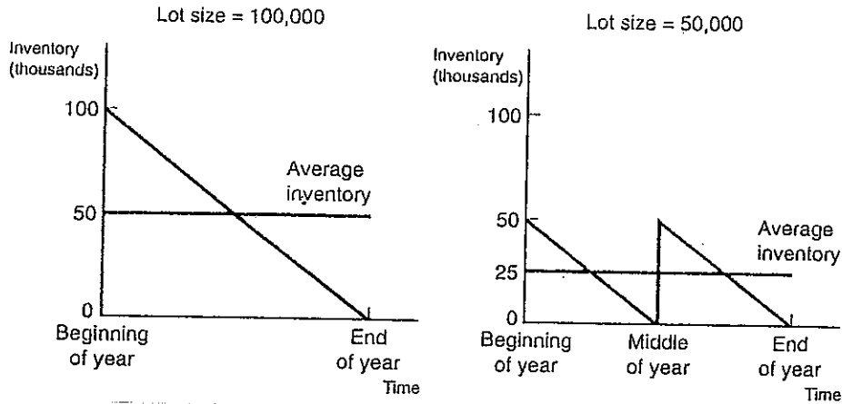
FIGURE 2. Size of Inventory During the Year, Given that Lot Size Equals 100,000 and 50,000. Average inventory is 50,000 parts if the lot size equals 100,000, and 25,000 parts if the lot size equals 50,000.
